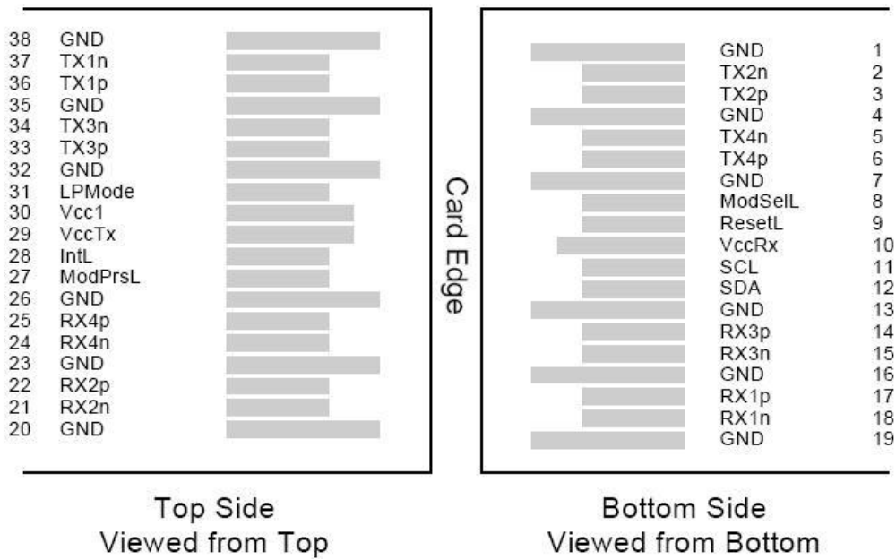
Figure 2. QSPF28 Transceiver Electrical Connector Layout
